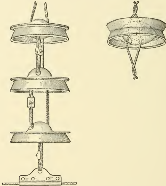
Fig. 40. Suspended or Disk Type of Insulator
